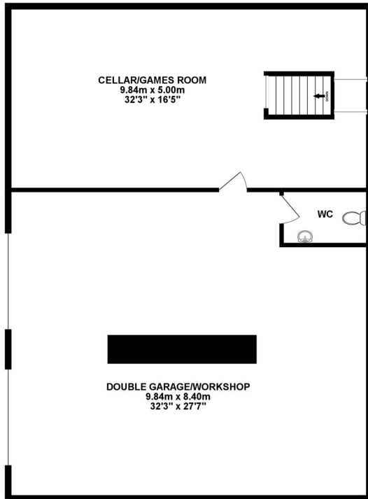
BASEMENT 131.84 sq. m. ( 1419.10 sq. ft. )
