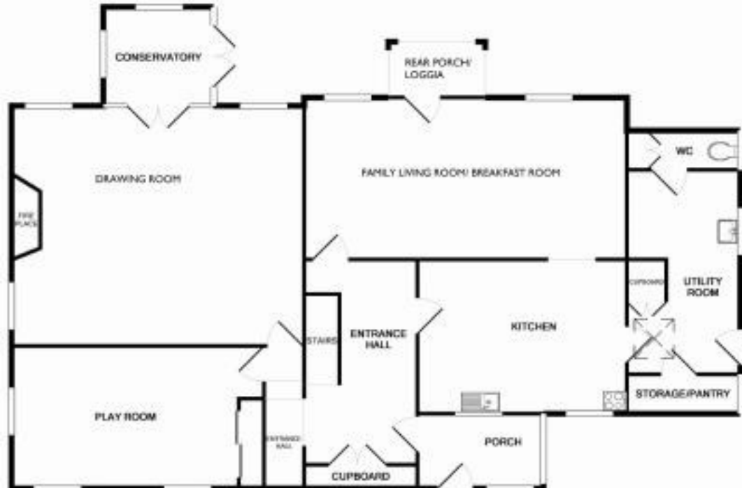
GROUND FLOOR
